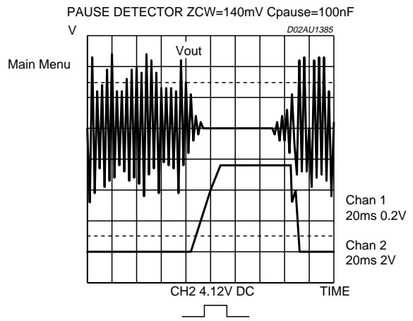
Figure 12. Pause Detector
